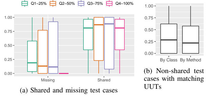
Figure 2: (a) Proportion of missing and shared test cases in 25 %, 50 %, 75 %, and 100 % of the projects in each ecosystem; (b) Proportion of non-shared test cases with matching UUTs in other projects of the ecosystem.
